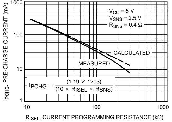
Figure 10. Pre-Charge Current versus Current Programming Resistor
