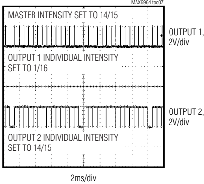
SCOPE SHOT OF OUTPUT PORTS
