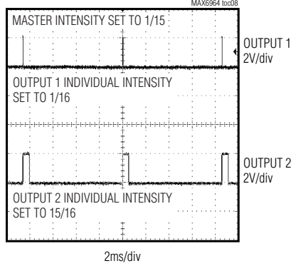
SCOPE SHOT OF OUTPUT PORTS
