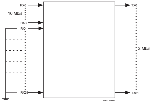
Figure 4. Mux/Demux Mode
