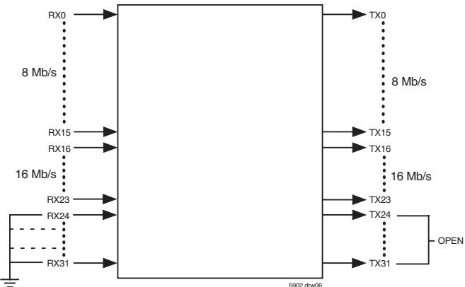
Figure 5. Split Mode
