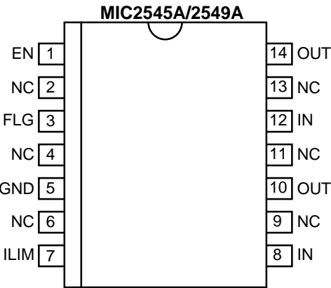
14-Lead TSSOP (TS)
