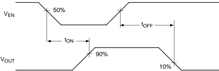
Figure 1a. MIC2545A/49A-2
