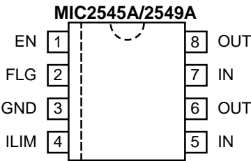
8-Lead SOP (M) 8-Pin DIP (N)
