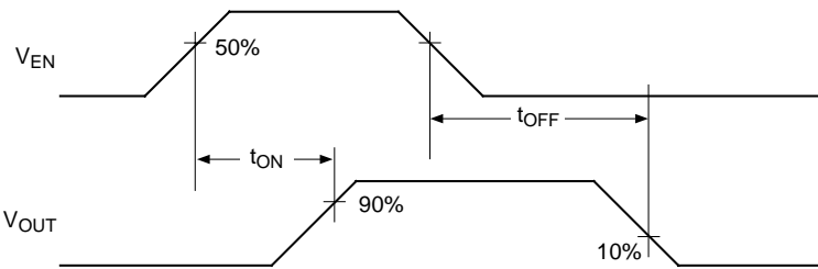
Figure 1b. MIC2545A/49A-1
