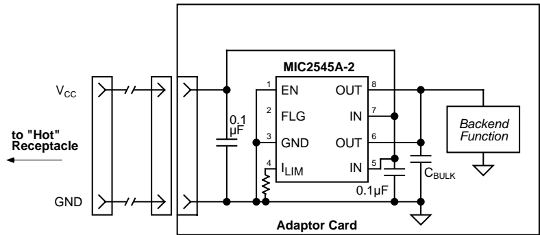
Figure 5. Hot-Plug Application
