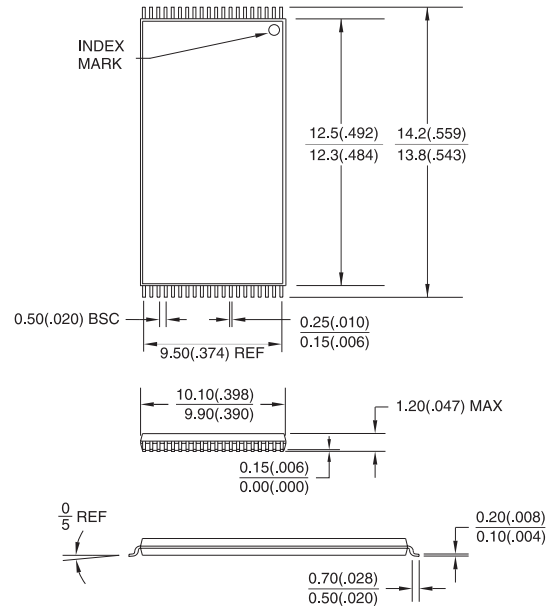
40V, 40-Lead, Plastic Thin Small Outline Package (VSOP) Dimensions in Millimeters and (Inches)*
