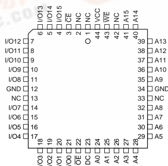
PLCC Top View
