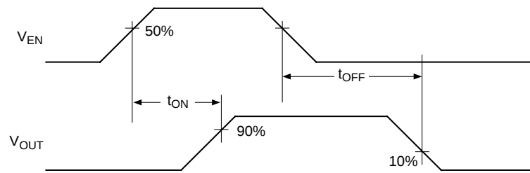
Figure 1a. MIC2546/47-1
