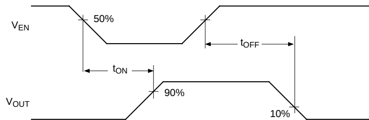
Figure 1b. MIC2546/47-2
