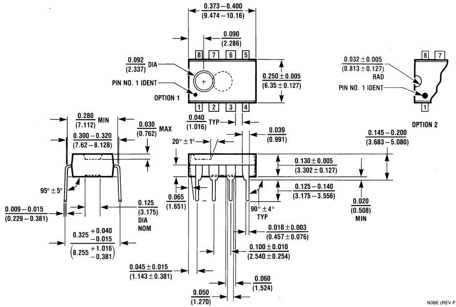
Order Number LM4881N NS Package Number N08E
