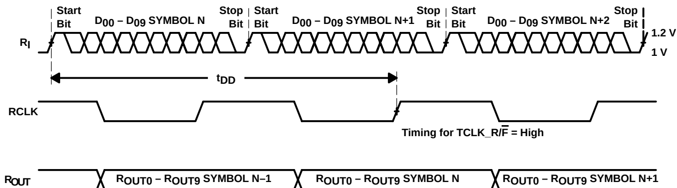
Figure 13. Deserializer Delay
