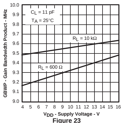
GAIN BANDWIDTH PRODUCT VS SUPPLY VOLTAGE
