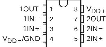
TLV2662M, TLV2262AM U PACKAGE (TOP VIEW)
