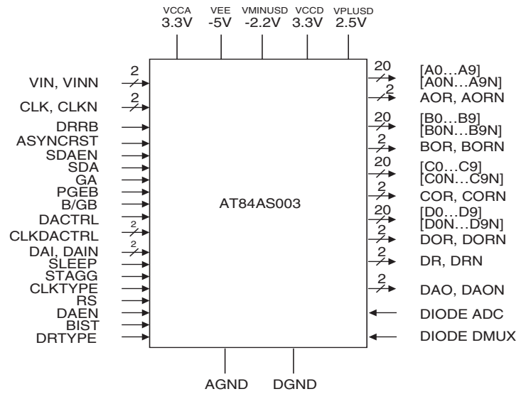
Figure 2. Device Pinout
