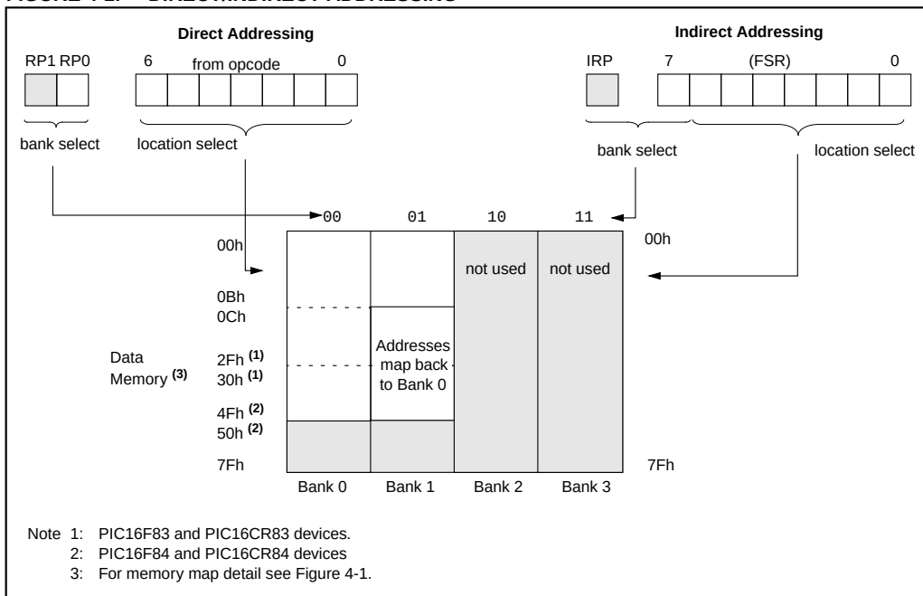
FIGURE 4-1: DIRECT/INDIRECT ADDRESSING
