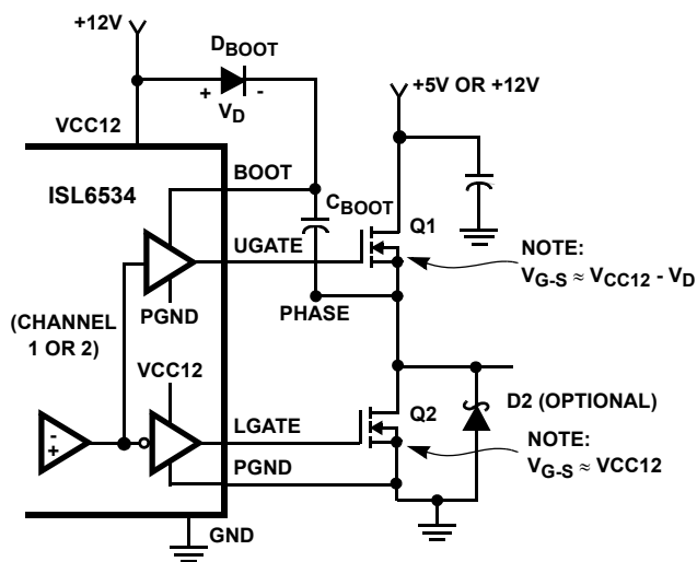
FIGURE 17. UPPER GATE DRIVE - BOOTSTRAP OPTION
