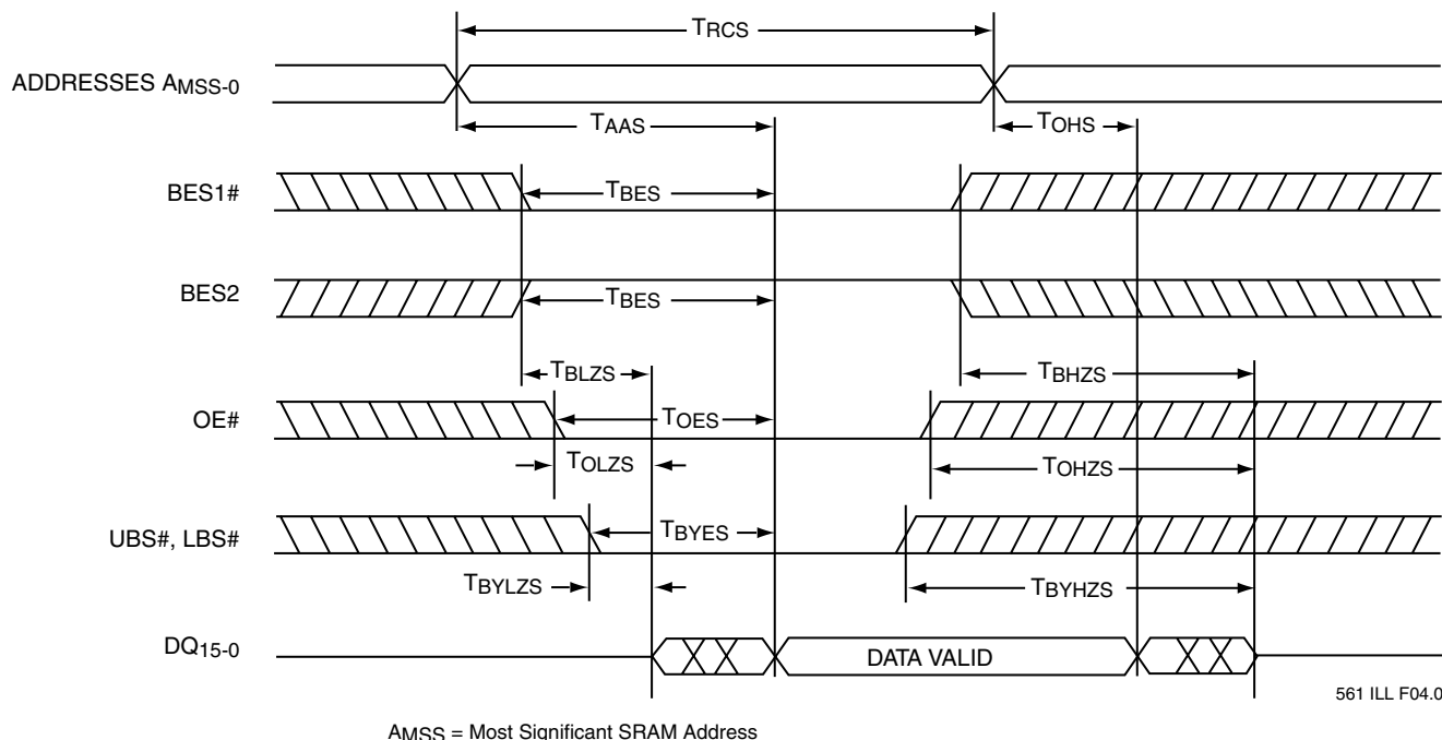
FIGURE 3: SRAM READ CYCLE TIMING DIAGRAM
