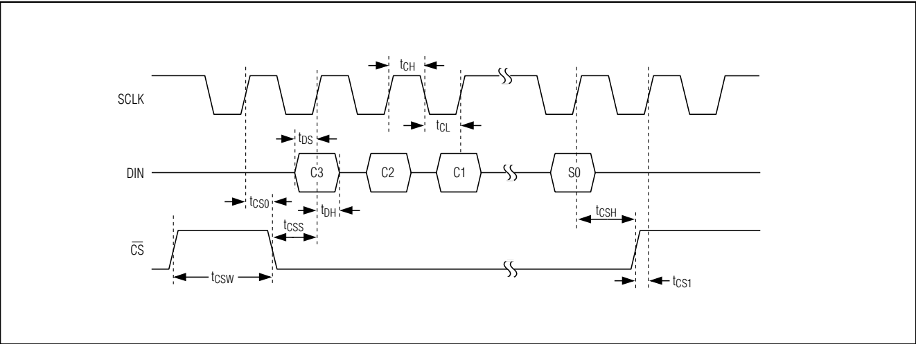
Figure 1. Timing Diagram
