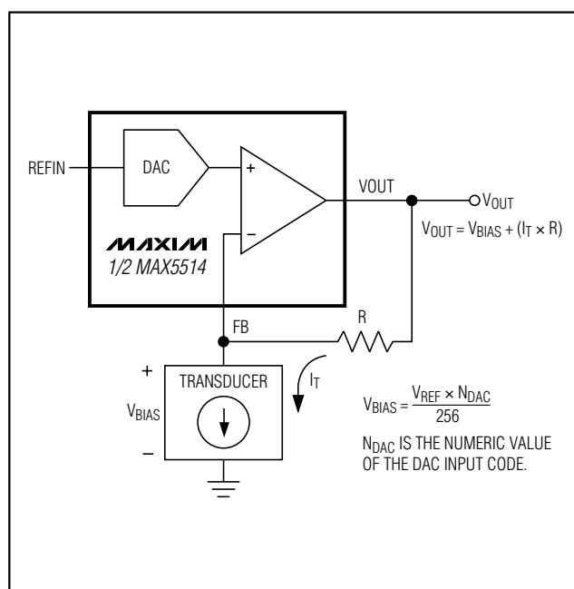
Figure 5. Transimpedance Configuration for a Voltage-Biased Current-Output Transducer
