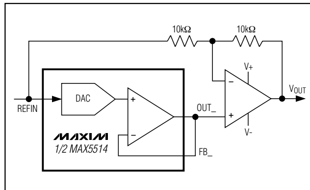
Figure 7. Bipolar Output Circuit
