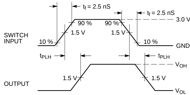
Figure 3. Propagation Delays
