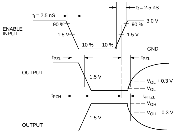
Figure 4. Enable/Disable Delays
