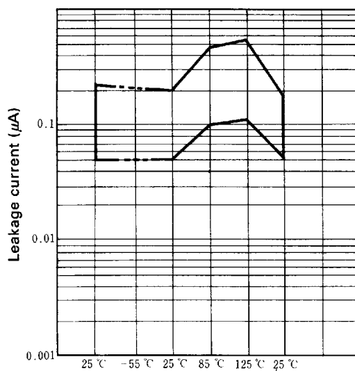
4 V/68 \mu F D case
