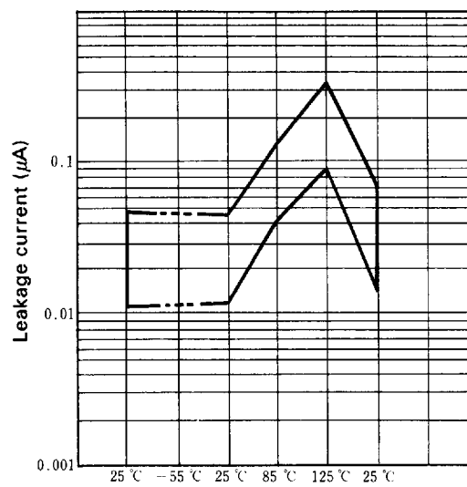
35 V/6.8 \mu F D case
