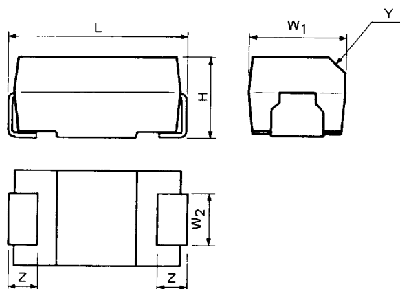
[B, C &amp; D cases]
