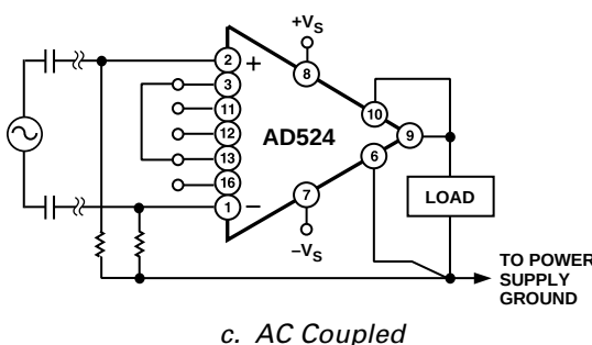
Figure 34. Indirect Ground Returns for Bias Currents
