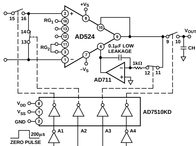
Figure 45. Autozero Circuit
