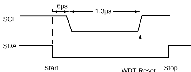
Figure 4. Watchdog Restart
