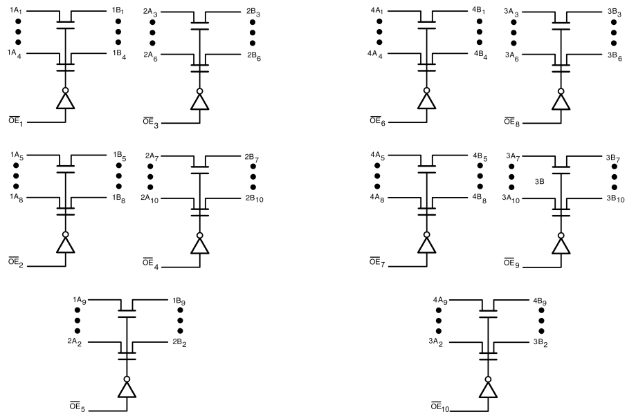
4-Bit Configuration
