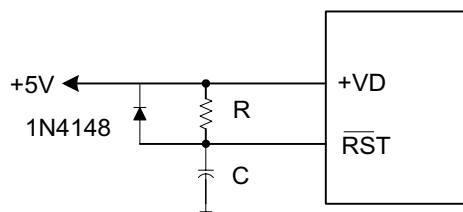
FIGURE 8. POWER-UP RESET CIRCUIT
