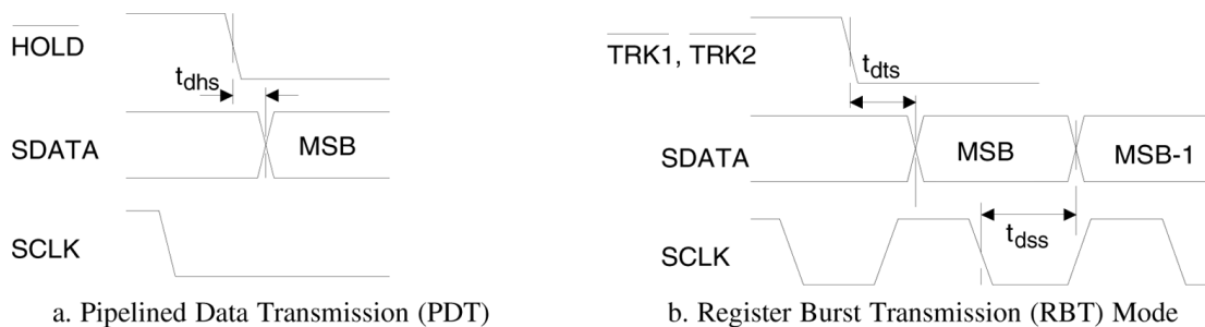
FIGURE 6. DATA TRANSMISSION TIMING
