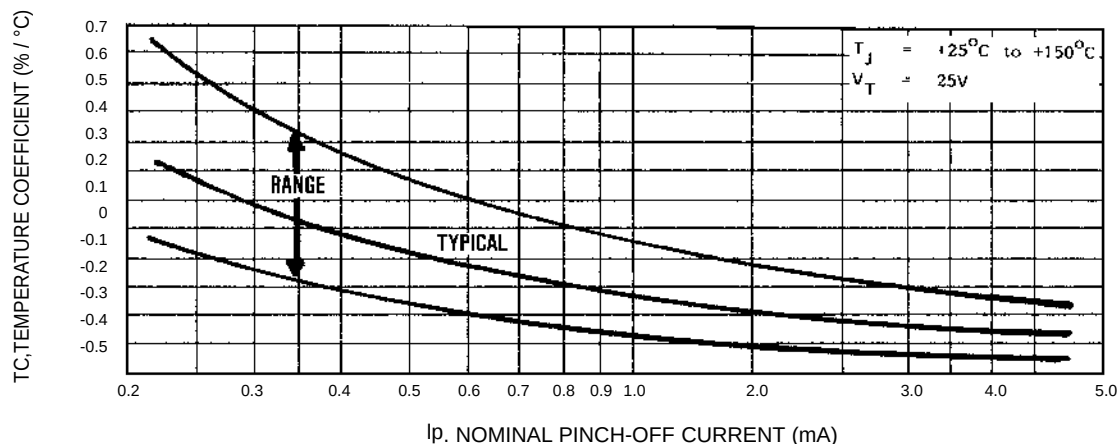
FIGURE 2 TEMPERATURE COEFFICIENT
