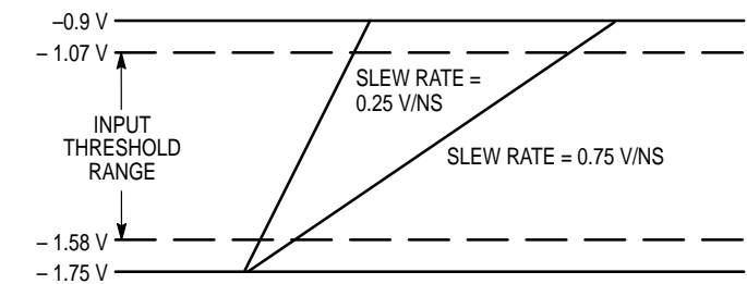
Figure 4. ECL Dispersion Test Input Conditions
