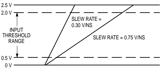
Figure 5. TTL Dispersion Test Input Conditions
