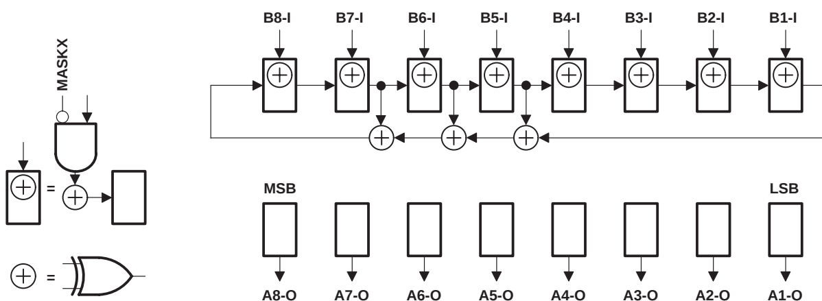
Figure 11. 8-Bit PSA/COUNT Configuration ( \overline{\text{OEAB}} = 1, \overline{\text{OEBA}} = 0 )
