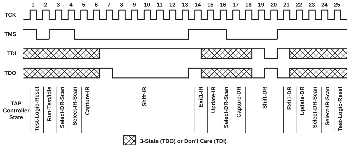
Figure 12. Timing Example
