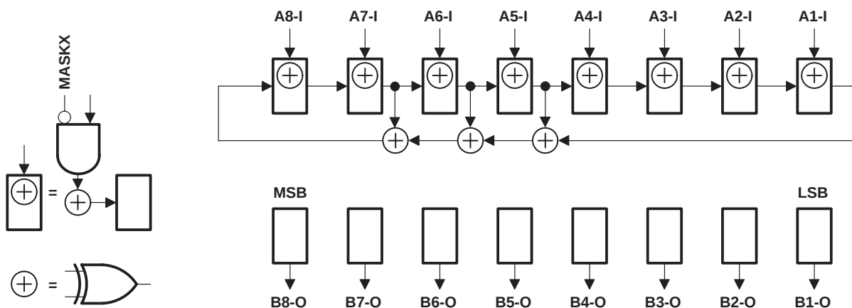
Figure 10. 8-Bit PSA/COUNT Configuration ( \overline{\text{OEAB}} = 0 , \overline{\text{OEBA}} = 1 )
