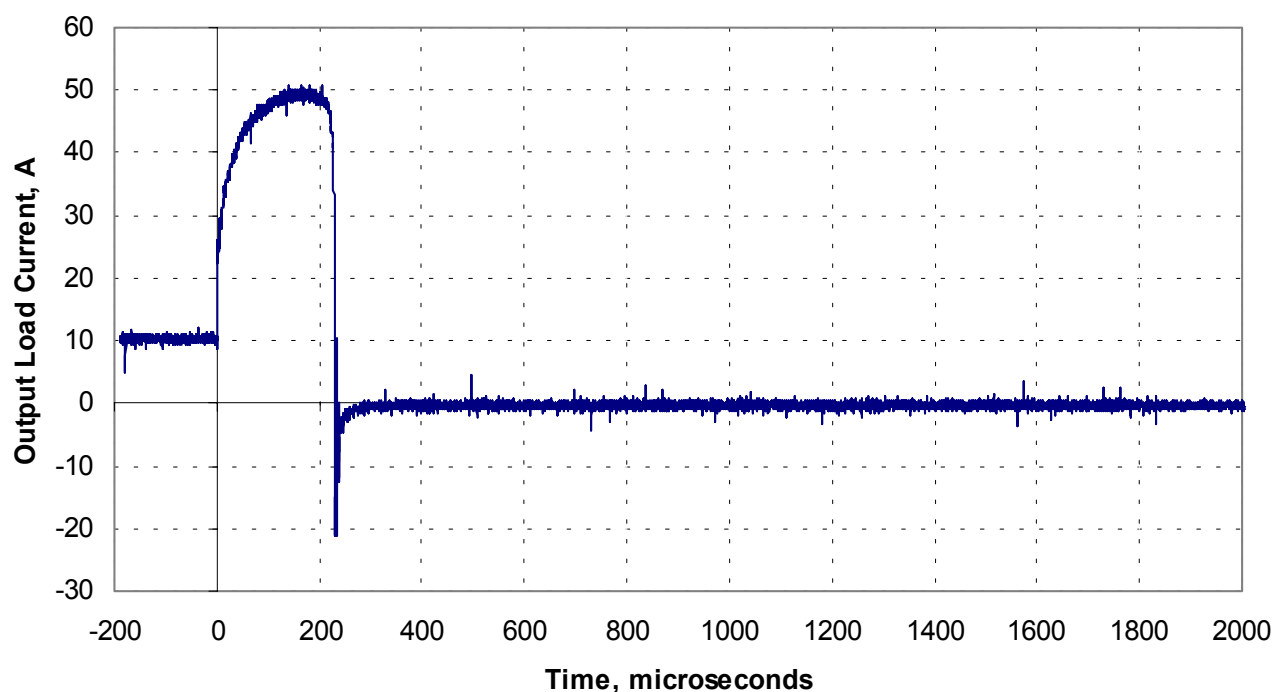
Typical Waveform 53248-102 Short Circuit Protection: Short-while-On @ 25°C
