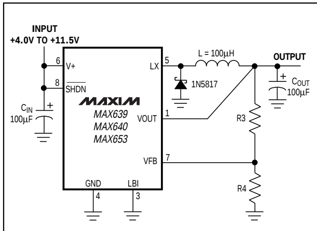
Figure 4. Adjustable-Output Operation
