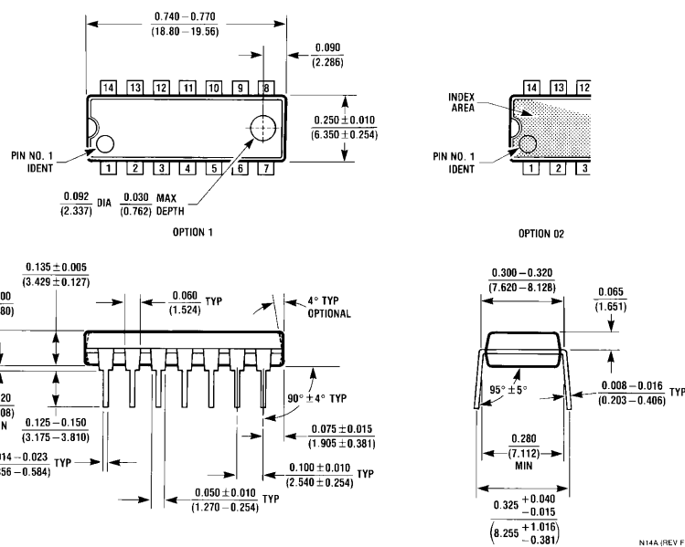
14-Lead Molded Dual-In-Line Package (N) Order Number DM7420N NS Package Number N14A
