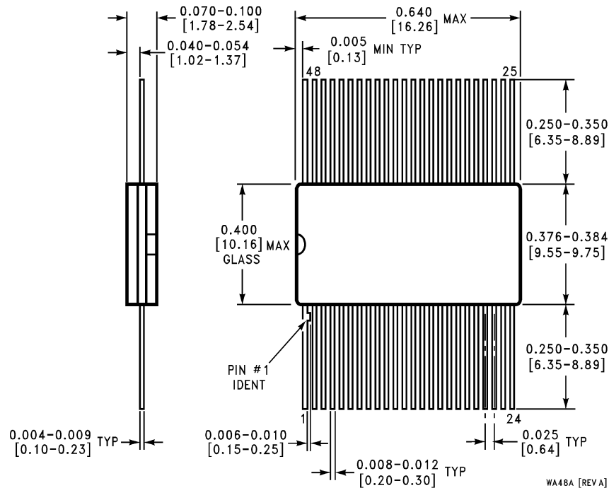
48-Lead Cerpack NS Package Number WA48A
