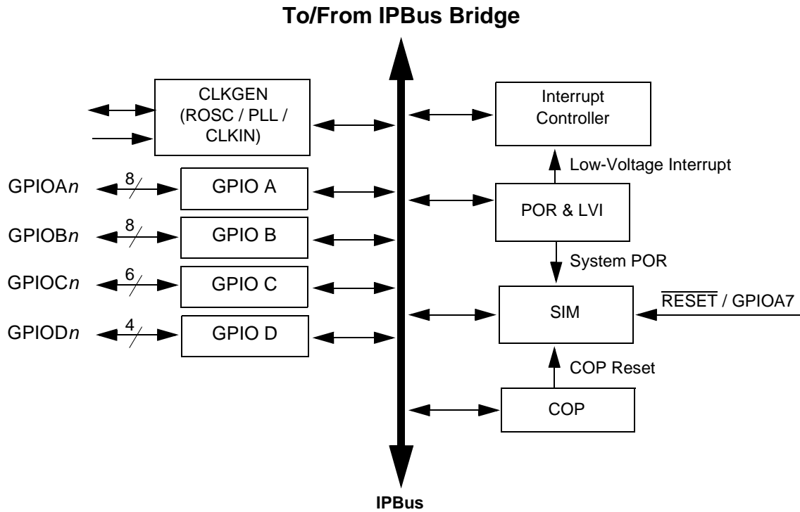
Figure 1-2 Peripheral Subsystem
