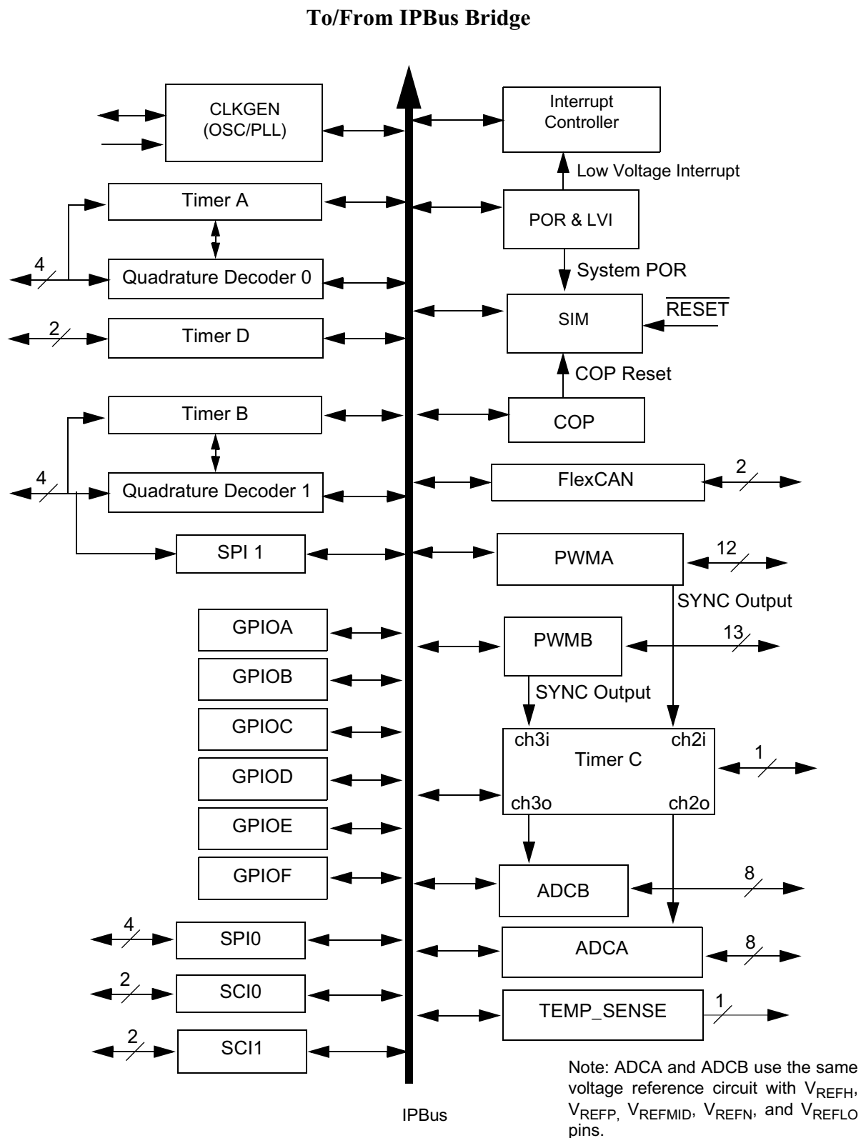
Figure 1-2 Peripheral Subsystem
