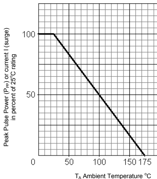
FIG. 4 Derating Curve
