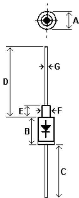
DO-13 (DO-202AA)
