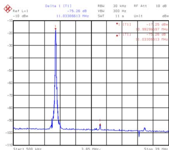
FIGURE 2. EDGE AT 11MHz, 78MSPS CLOCK (75dBc - NYQUIST, 6dB PAD)
