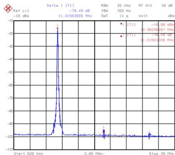
FIGURE 4. GSM AT 11MHz, 78MSPS CLOCK (78dBc - NYQUIST, 9dB PAD)
