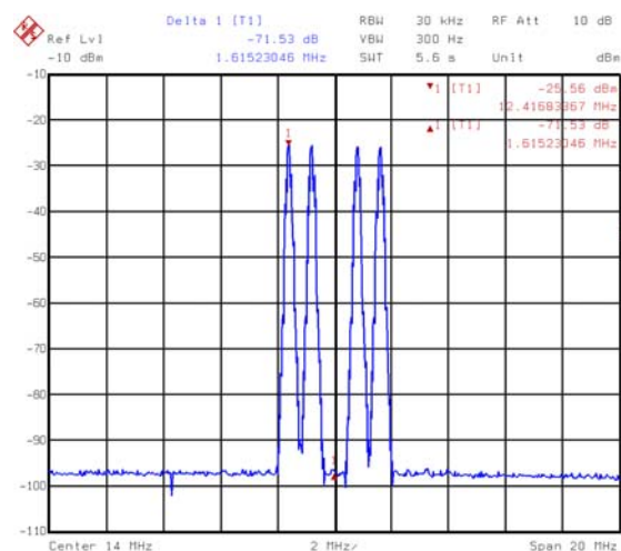
FIGURE 6. FOUR GSM CARRIERS AT 12.4-15.6MHz, 78MSPS (71dBc - 20MHz WINDOW, 6dB PAD)
