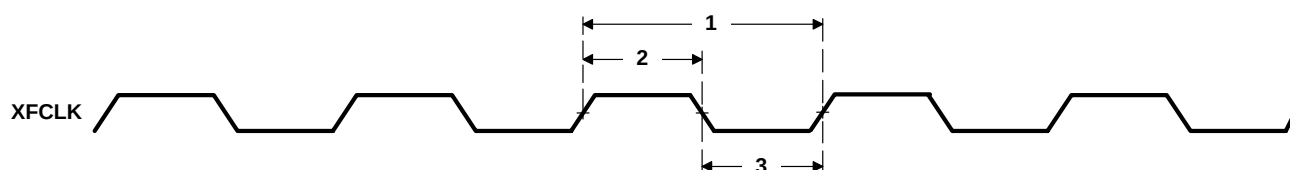
Figure 14. XFCLK Timings
