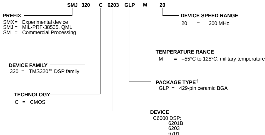
Figure 4. SMJ320C6000™ DSP Platform Device Nomenclature
