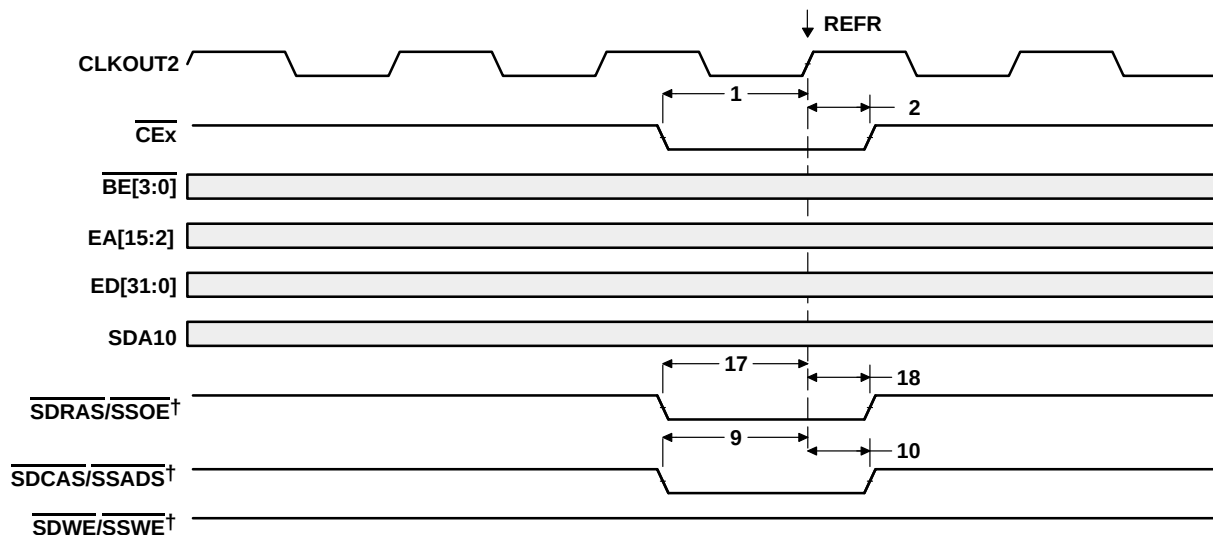
Figure 25. SDRAM REFRESH Command
