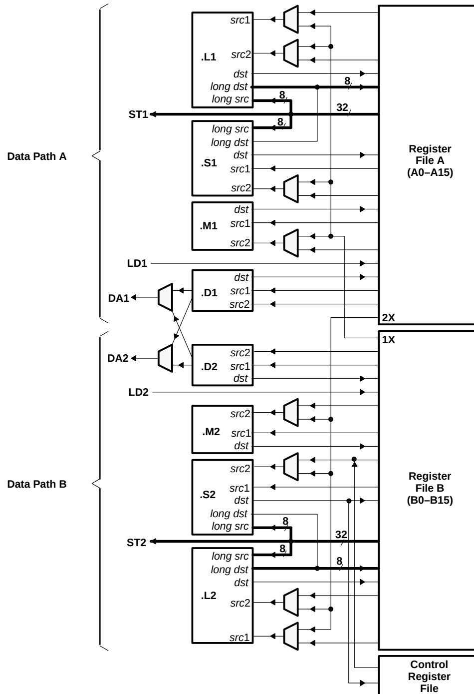
Figure 1. SMJ320C62x CPU (DSP Core) Data Paths
