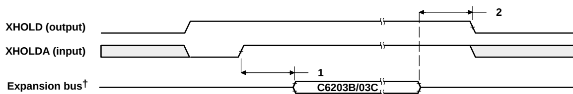
Figure 45. Expansion Bus Arbitration—Internal Arbiter Disabled
