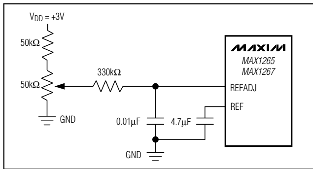
Figure 7. Reference Adjustment with External Potentiometer
