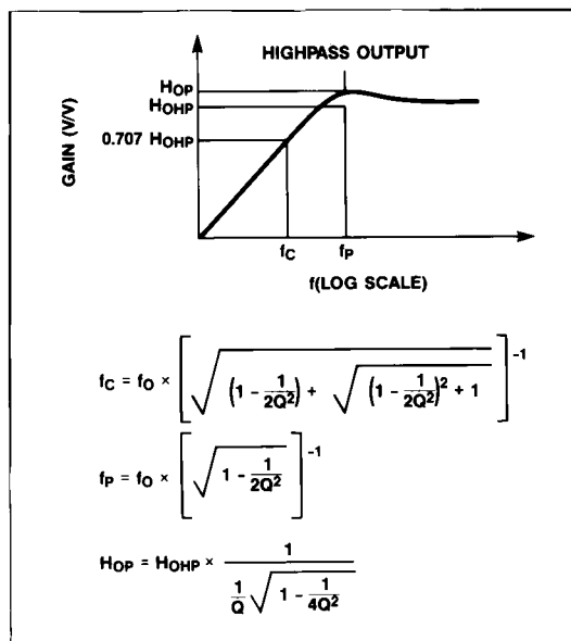
Figure 4. Highpass Response
