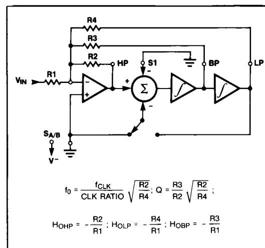
Figure 13. Mode 3: 2nd-Order Filter Providing Highpass, Bandpass, Lowpass
