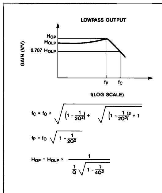
Figure 3. Lowpass Response
