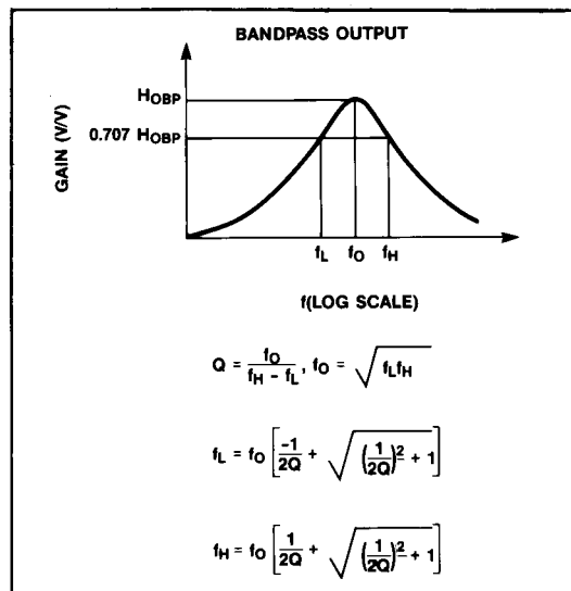
Figure 2. Bandpass Response
