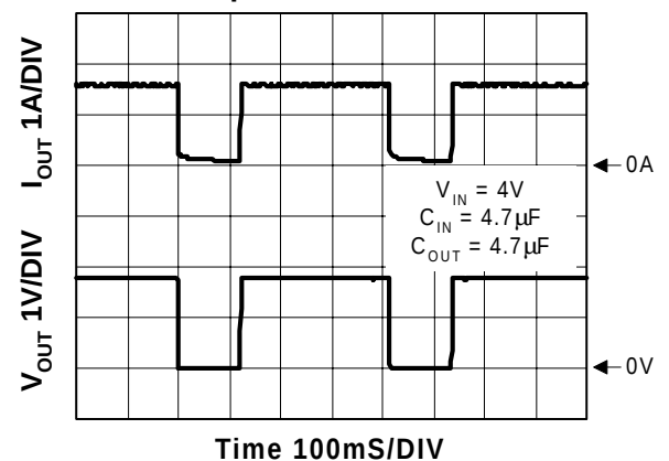
Overtemperature Shutdown
