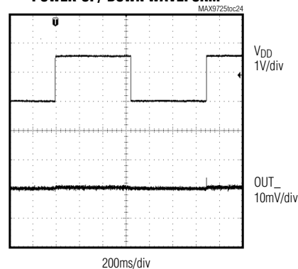
POWER-UP/-DOWN WAVEFORM
