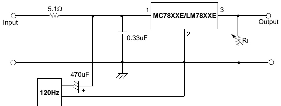
Figure 7. Ripple Rejection
