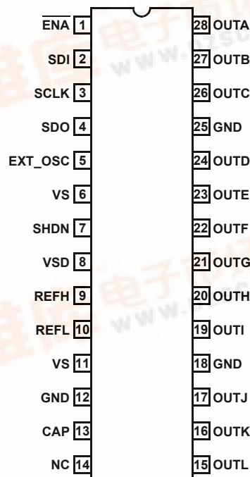
EL5325A (28-PIN TSSOP) TOP VIEW
