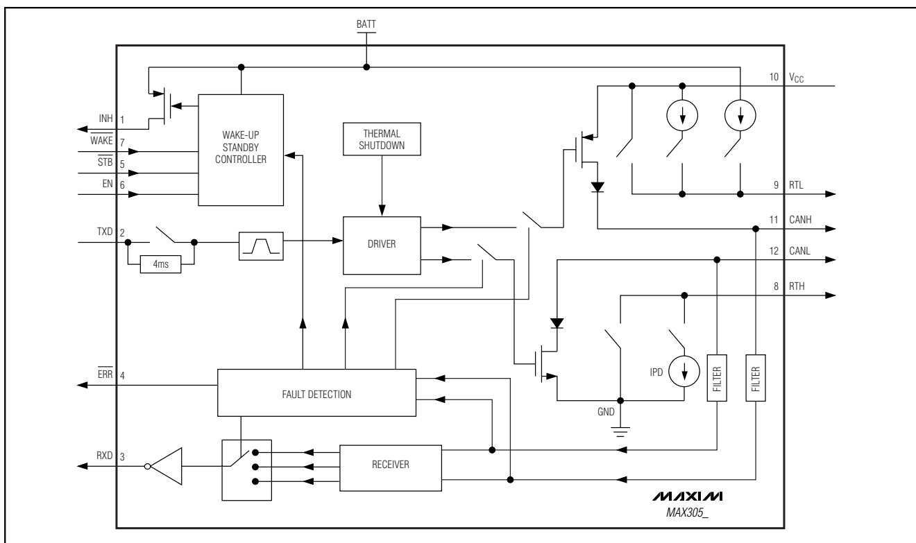
Figure 5. Block Diagram
