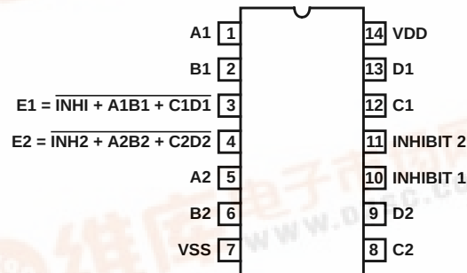
CD4085BMS TOP VIEW
