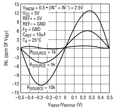
Figure 25. INL vs Differential Input Voltage ( V_{IN} = IN^+ - IN^- ) and Reference Source Resistance ( R_{SOURCE} ) at REF^+ and REF^- for Large C_{REF} Values ( C_{REF} \geq 1\mu\text{F} )
