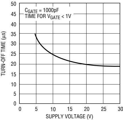
Turn-OFF Time
