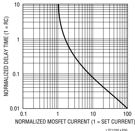
Figure 5. Normalized Delay Time vs MOSFET Current
