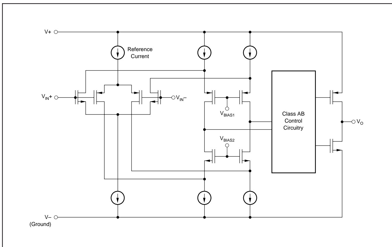
FIGURE 2. Simplified Schematic.
