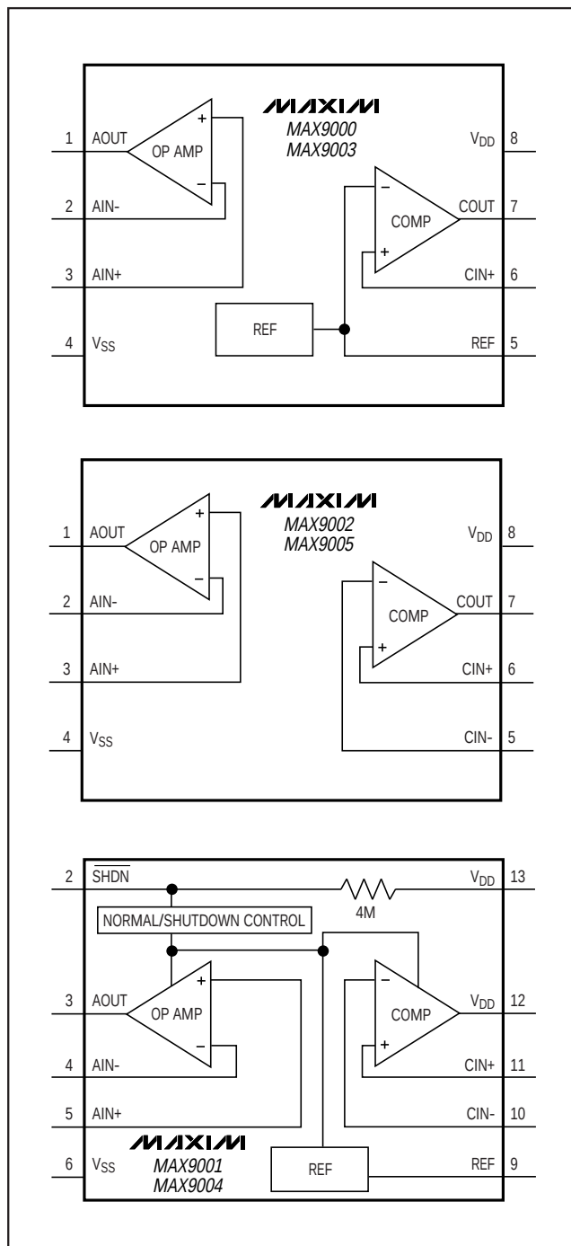
Figure 1. MAX9000–MAX90005 Functional Diagrams
