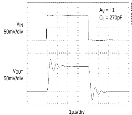
MAX9000/MAX9001/MAX9002 OP-AMP SMALL-SIGNAL TRANSIENT RESPONSE WITH C LOAD
