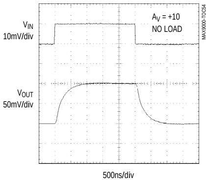
MAX9003/MAX9004/MAX9005 OP-AMP SMALL-SIGNAL TRANSIENT RESPONSE
