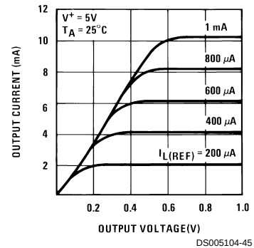
Output Characteristics
