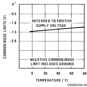
Common-Mode Limits
