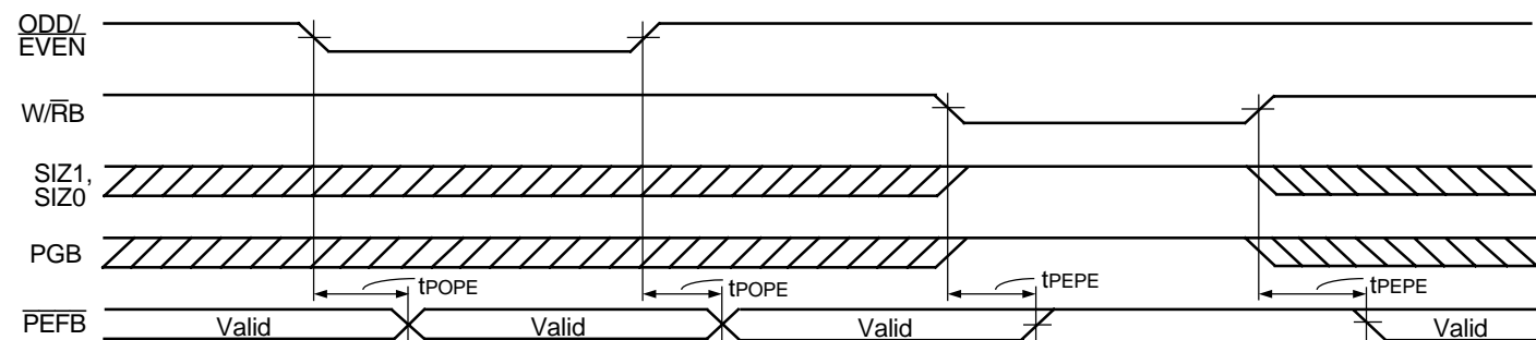
Figure 17. ODD/ \overline{EVEN} , W/ \overline{RB} , SIZ1, SIZ0, and PGB to \overline{PEFB} Timing
