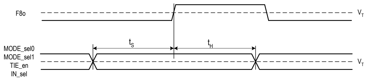
Figure - 14 Input Control Setup and Hold Timing
