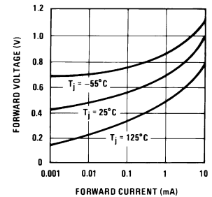
Forward Characteristics
