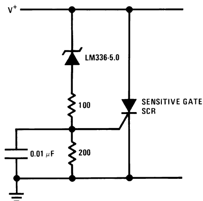
5V Crowbar
